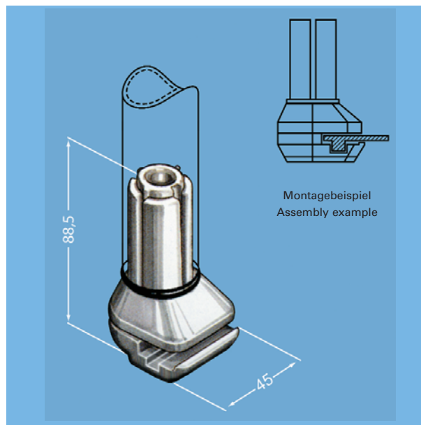
606 0063 Side-wall/Floor Bearing
