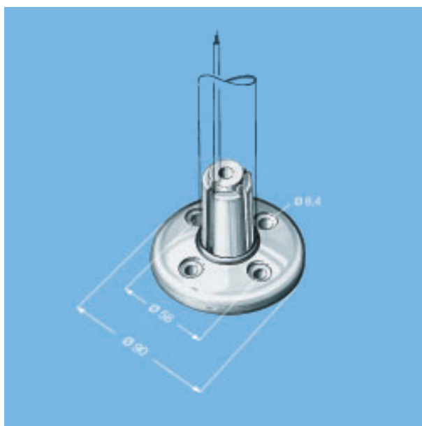
606 0080 Floor Bearing
