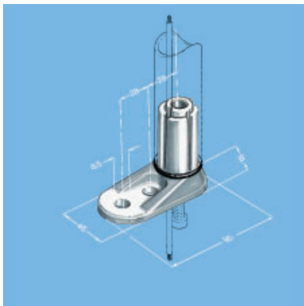
606 0062 Floor Bearing
